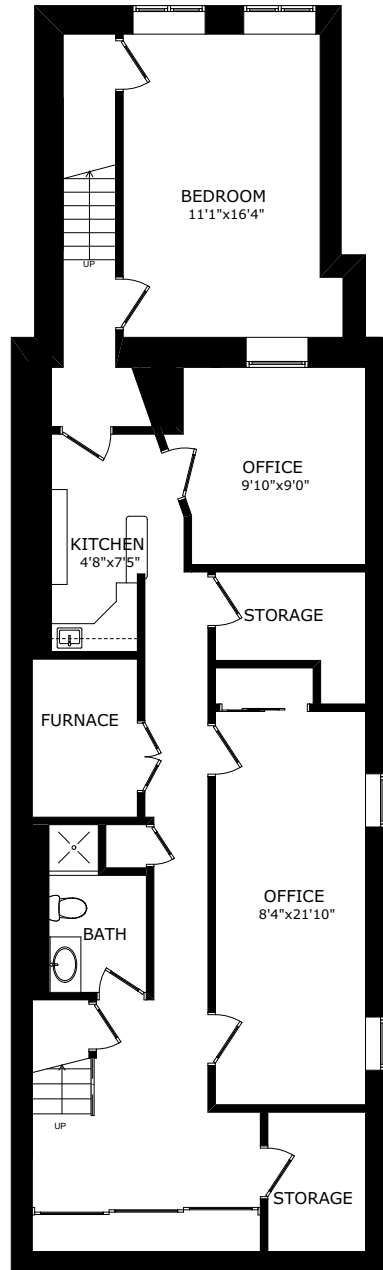
BASEMENT
