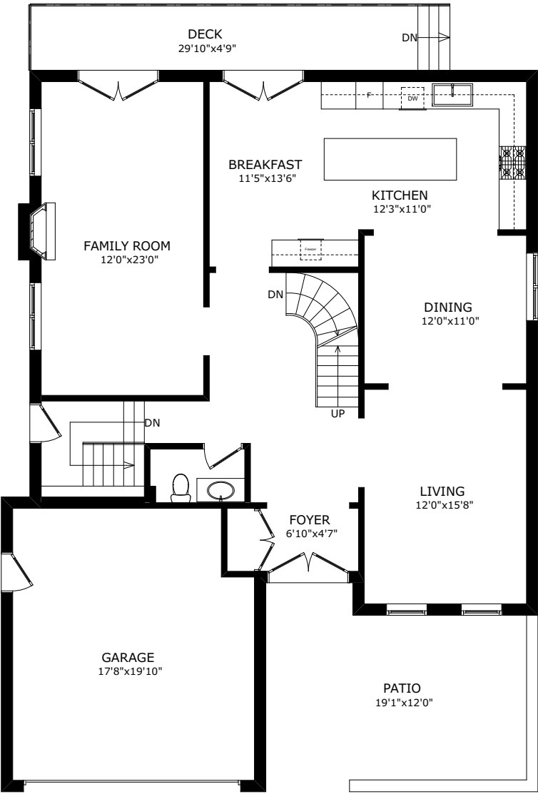
MAIN FLOOR
