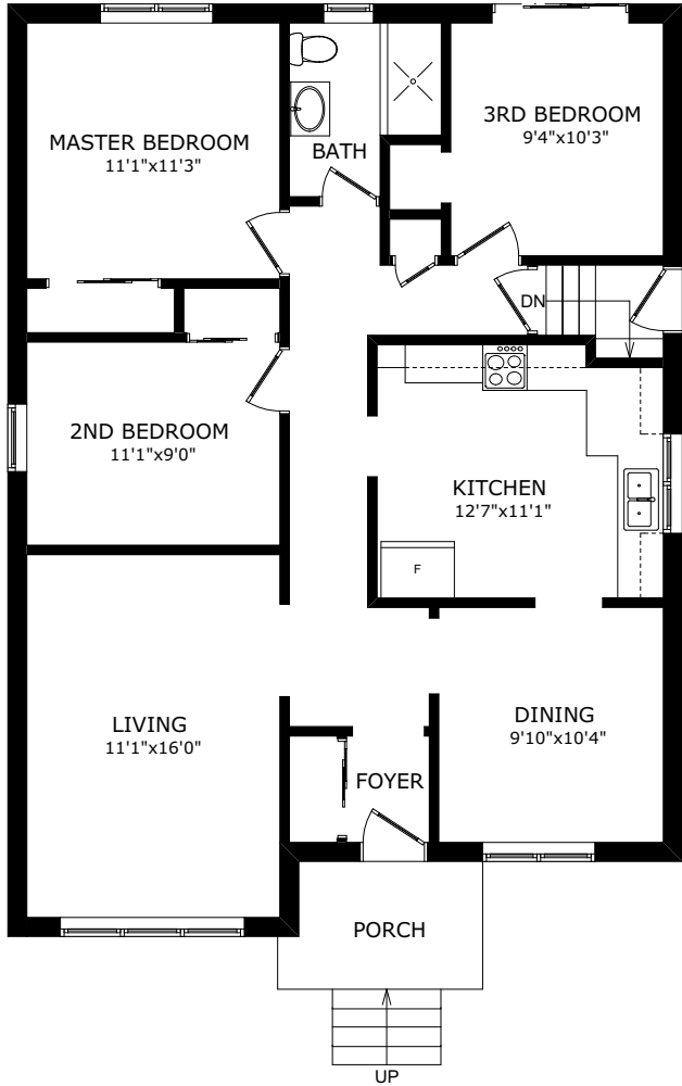
MAIN FLOOR
